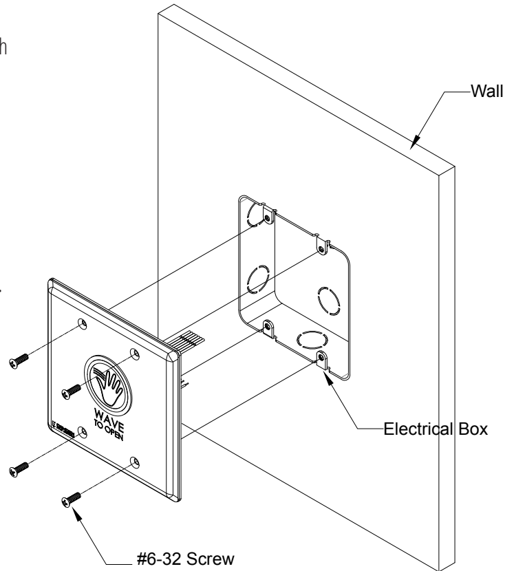
Figure 4.5.2 Single Gang Installation
