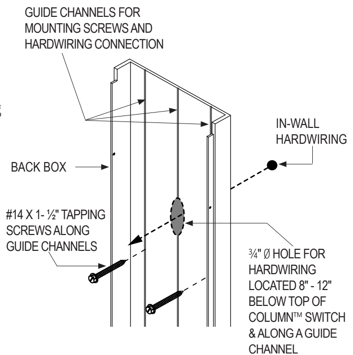
Figure 9.2 Guide Channels
