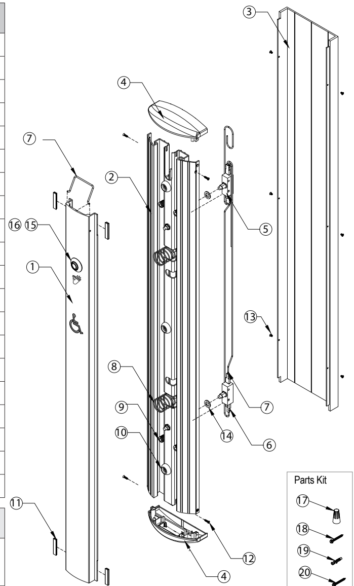
Figure 12.1 Exploded View
