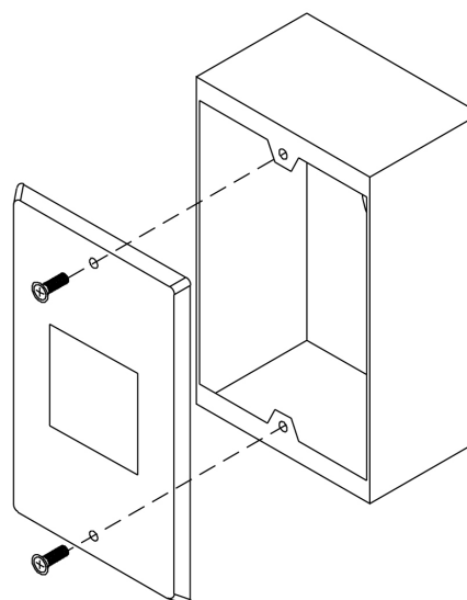
Figure 4.1 Installation
