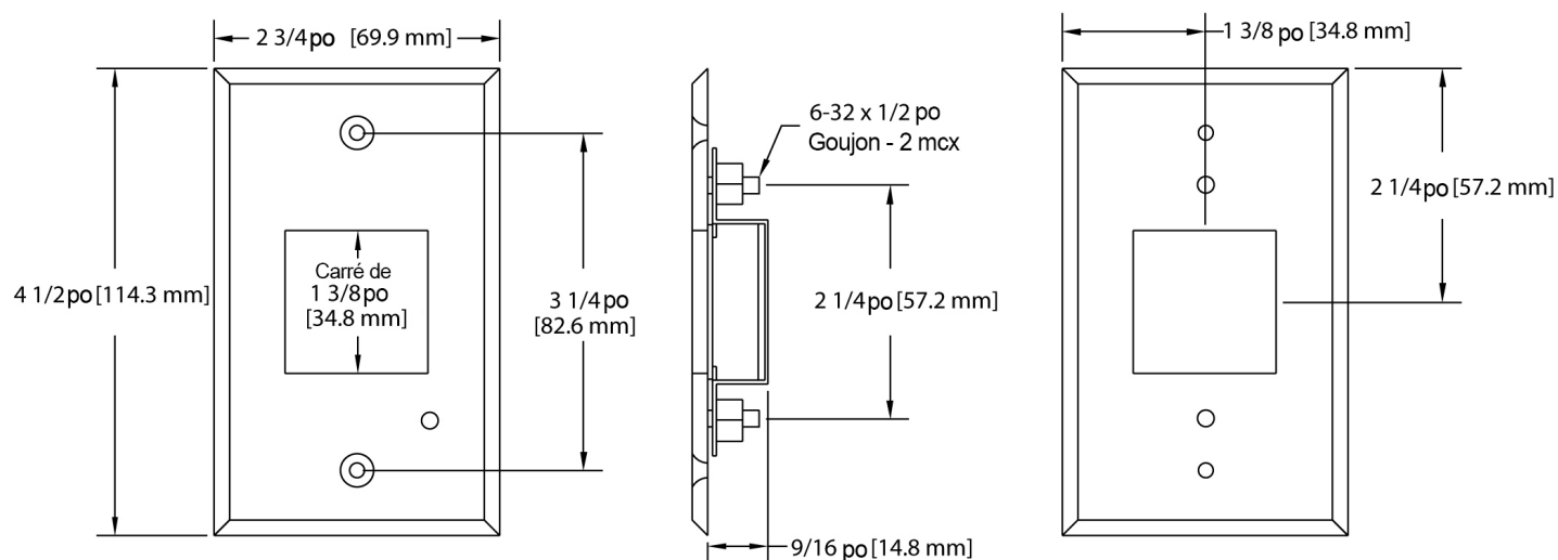
Figure 8.1 Dimensions
