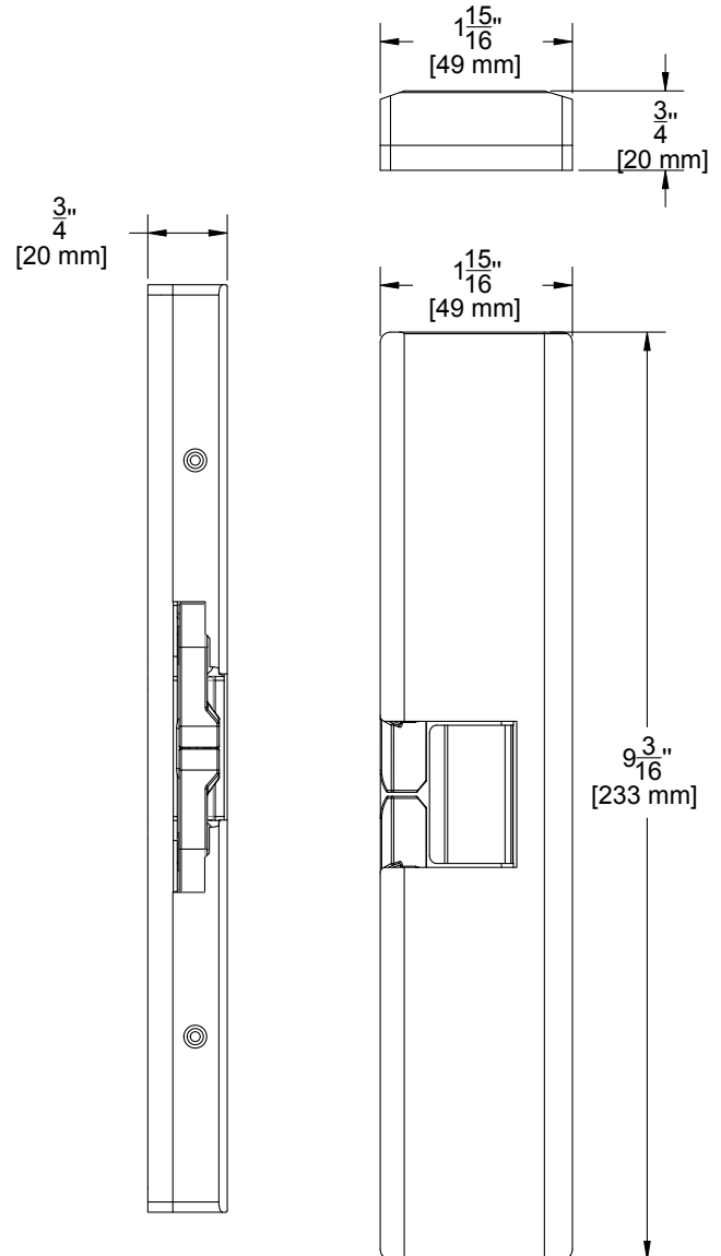
Figure 3.1 Dimensions
