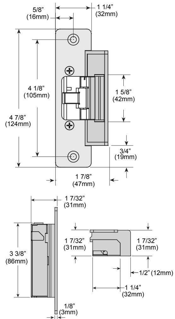
Figure 3.1 Dimensions
