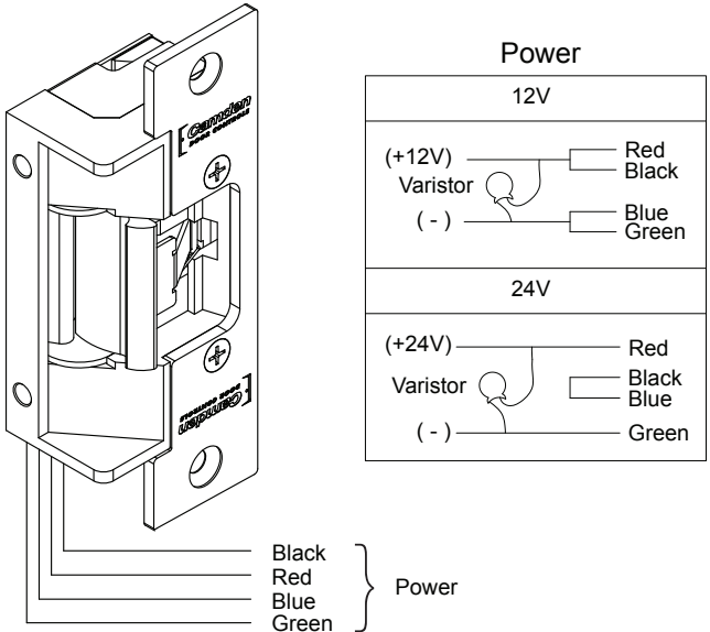
Figure 7.1 Connections for CX-ED2079
