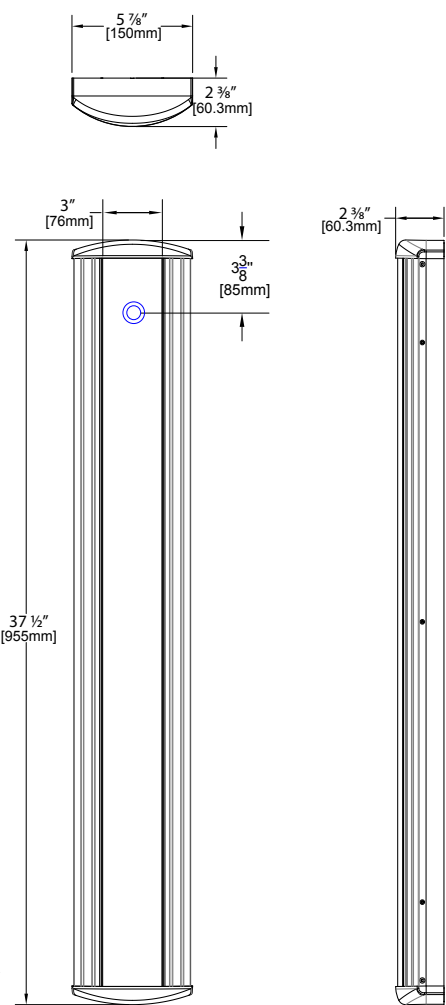
Figure 4.7 Dimensions
