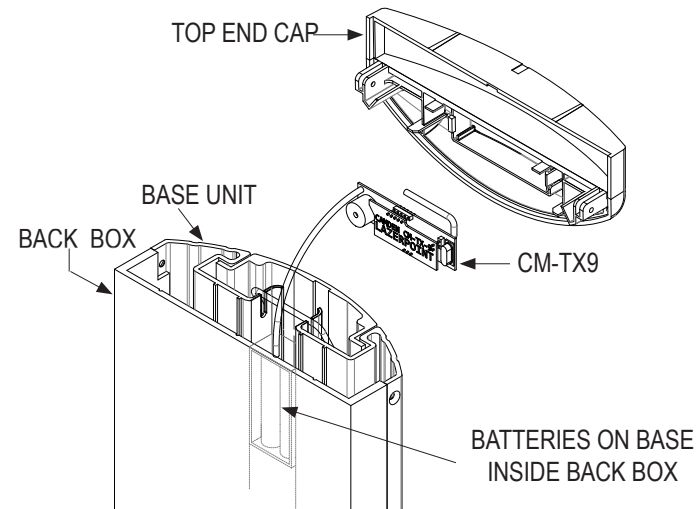
Figure 4.5 Transmitter Assembly
