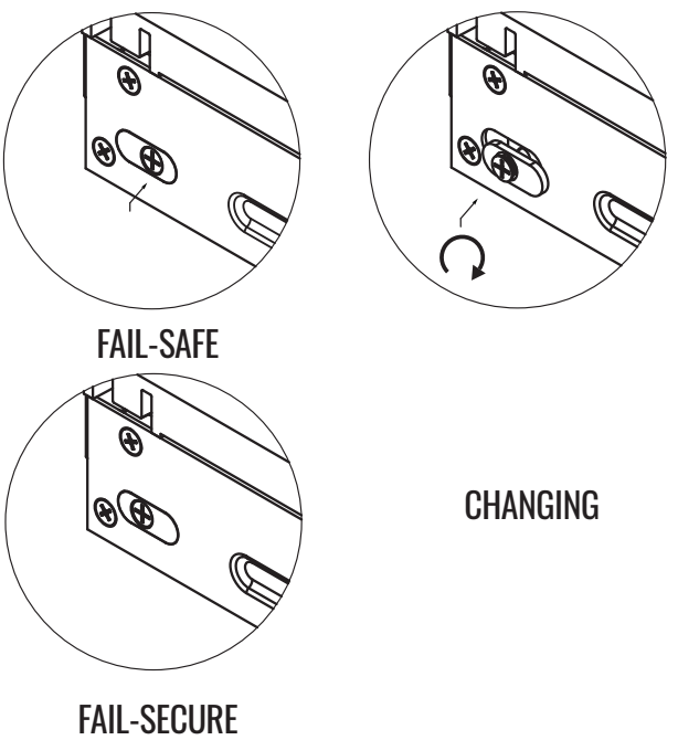
Figure 8.1 Fail Safe and Fail Secure Mechanism for CX-ED2079
