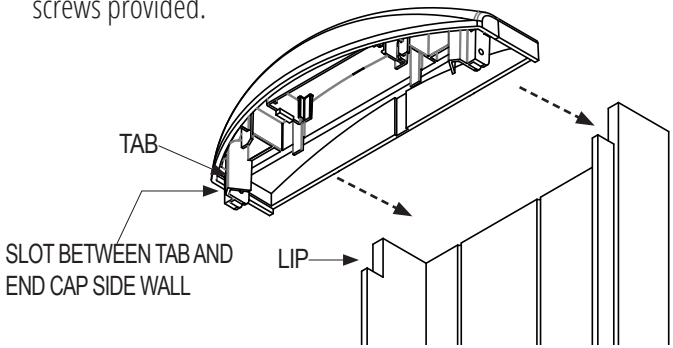
Figure 4.6 End Cap Alignment
