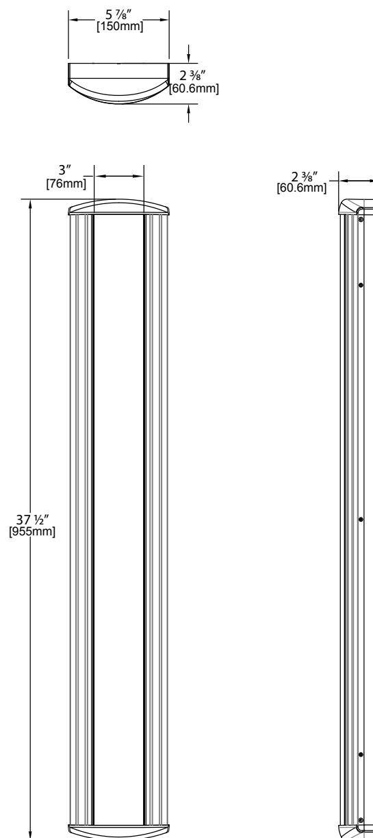
Figure 3.1 Dimensions
