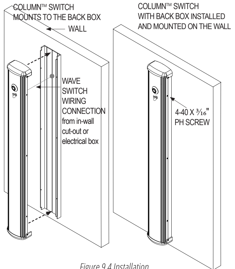
Figure 9.4 Installation
