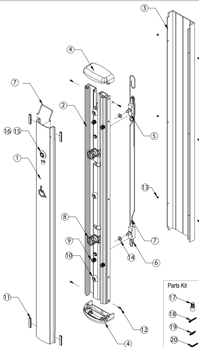
Figure 12.1 Exploded View
