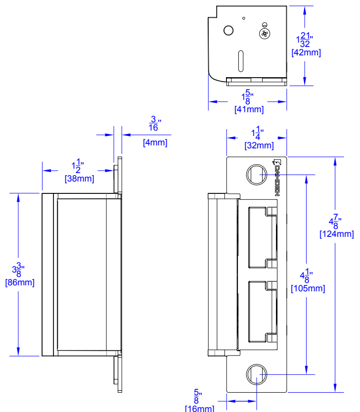
Figure 3.1 Dimensions
