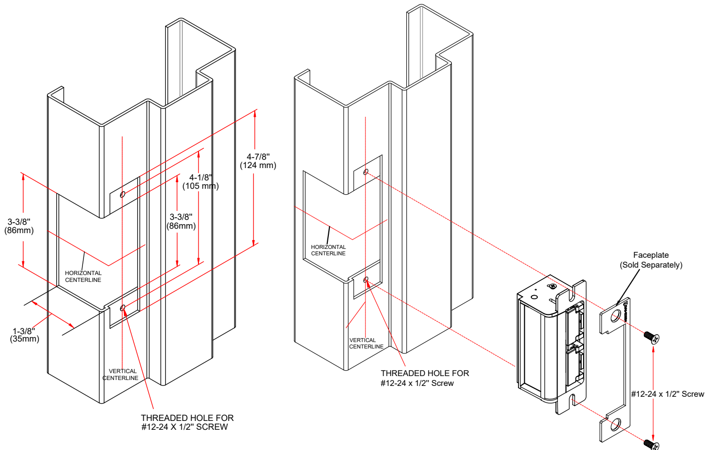
Figure 4.2 Cutout dimensions
