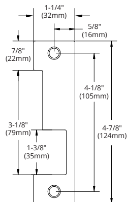
CX-EMP-6: For Sargent 8100/7700, Schlage and Yale mortise locksets
