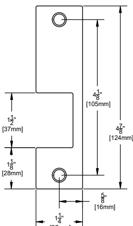
CX-EMP-2: Stainless faceplate for Arrow, Corbin & Best mortise locksets
