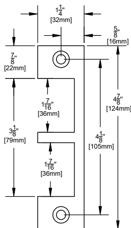
CX-EMP-5: Stainless faceplate for all mortise locks that include both latch & deadbolt
