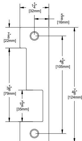
CX-EMP-6: Stainless faceplate for Sargent 8100/7700, Schlage, Yale 8700 locksets
