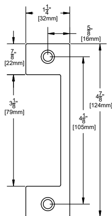
CX-EMP-4: Stainless faceplate for mortise locksets with deadbolt
