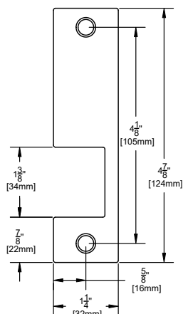
CX-EMP-1: Stainless faceplate for Sargent, Schlage & Yale mortise locksets
