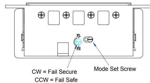
Figure 6.6 Strike operation from Fail Secure to Fail Safe and vice-versa
