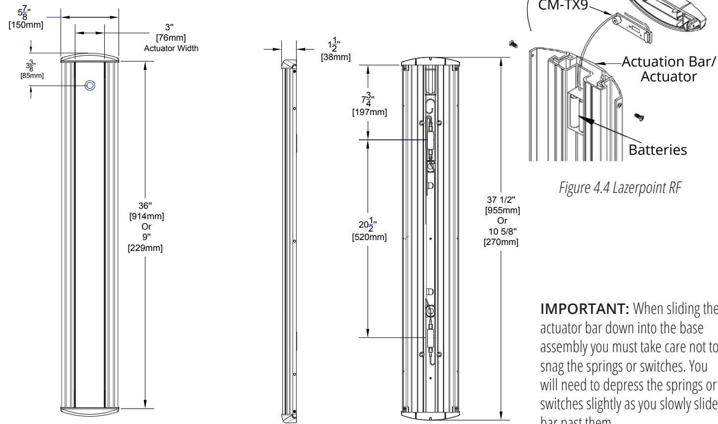
Figure 4.3 Dimensions
