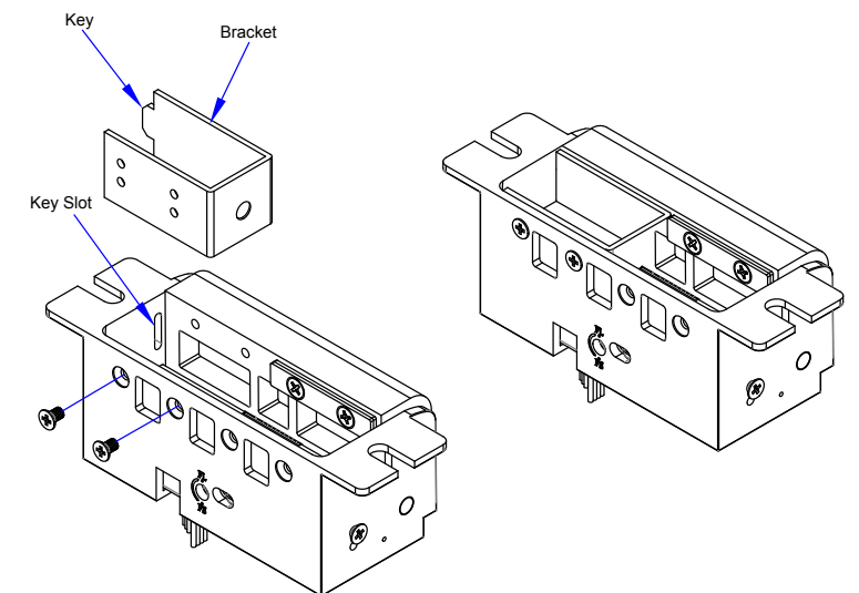
Figure 6.4 Deadbolt bracket installation
