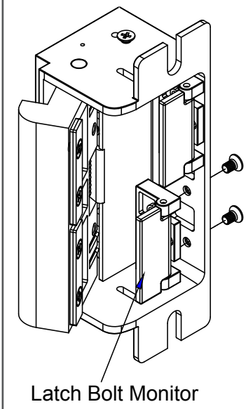
Figure 6.1 Latch bolt installation
