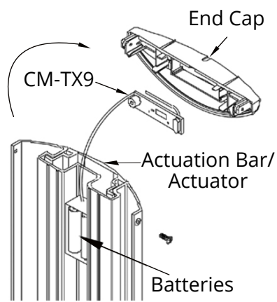
Figure 4.4 Lazerpoint RF
