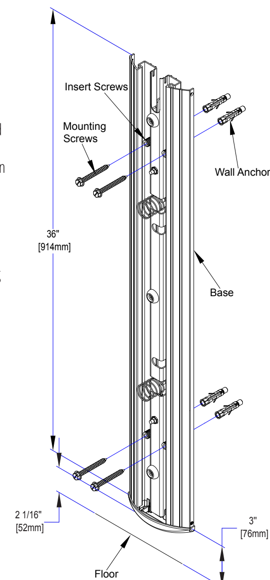
Figure 4.2 Mounting of Base Unit
