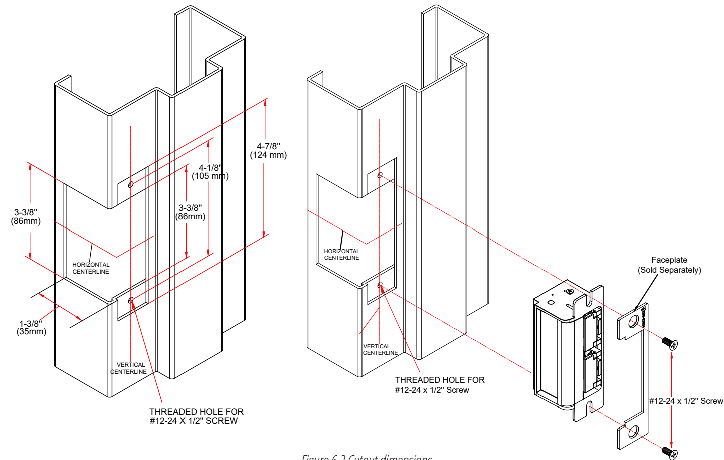
Figure 6.2 Cutout dimensions
