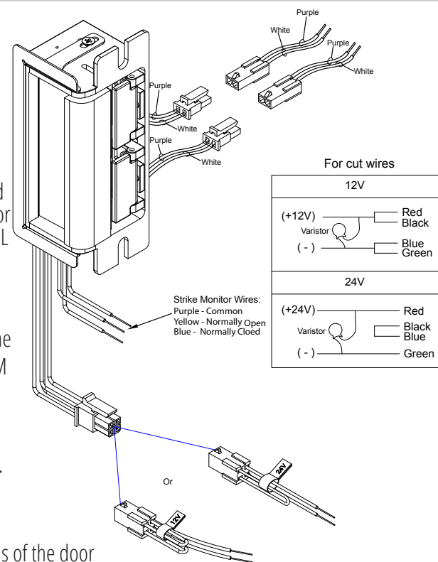
Figure 6.5 Bolt connection options
