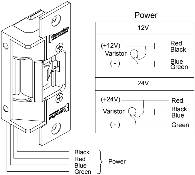
Figure 8.1 Connections for CX-ED2079
