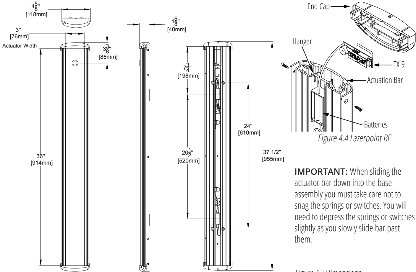
Figure 4.3 Dimensions
