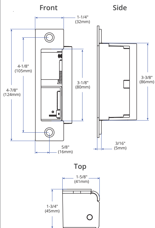
CX-EMP-1: For Sargent, Schlage and Yale mortise locksets
