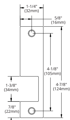
CX-EMP-1: For Sargent, Schlage and Yale mortise locksets
