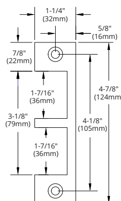
CX-EMP-5: For Arrow, Corbin and Best mortise locksets
