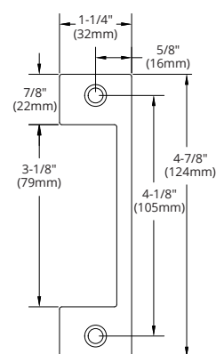
CX-EMP-4: For Sargent, Schlage and Yale mortise locksets
