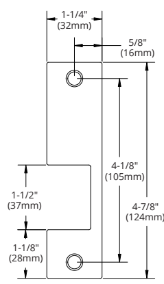
CX-EMP-2: For Arrow, Corbin and Best mortise locksets
