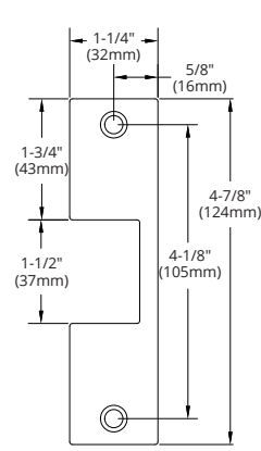
CX-EMP-3: For centerline mortise or cylindrical locksets
