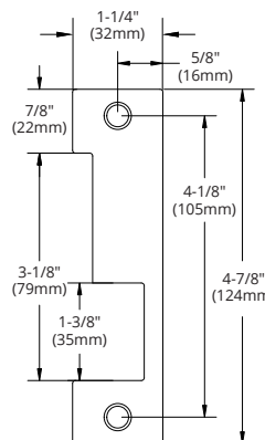
CX-EMP-6: For Sargent 8100/7700, Schlage and Yale mortise locksets
