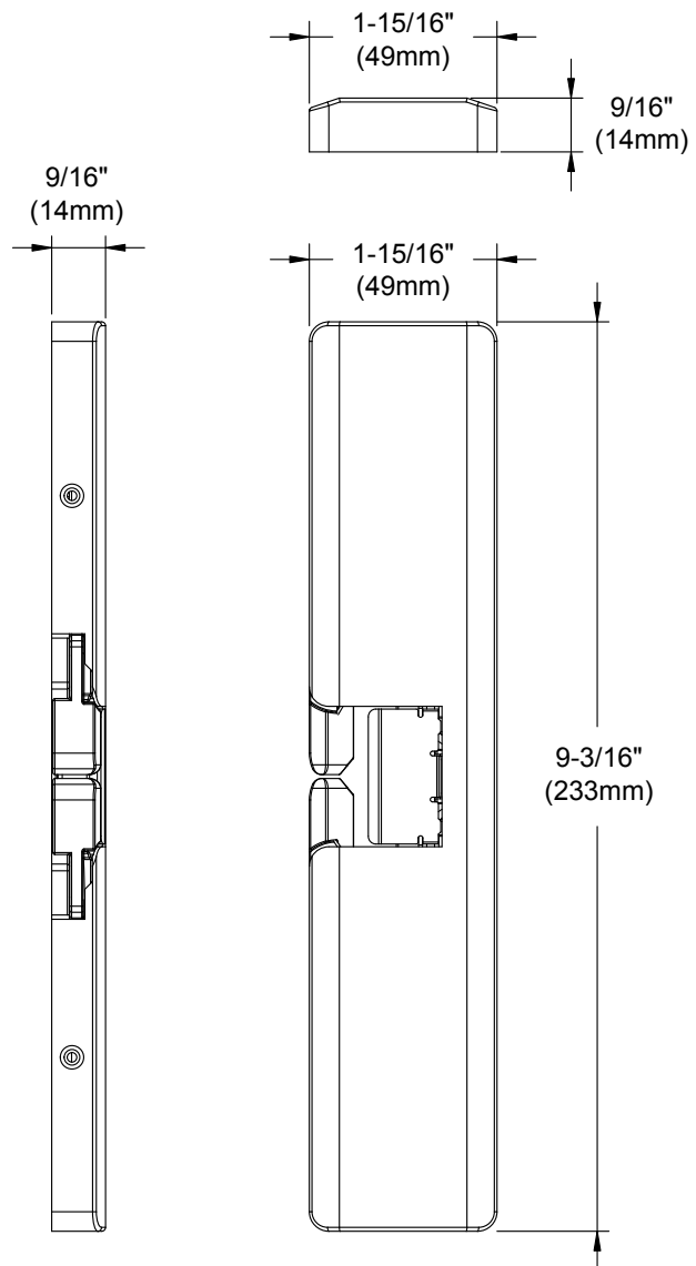
Figure 3.1 Dimensions
