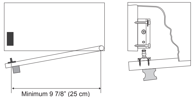
Illustrator 7: Mounting to a Fitted Cupboard
